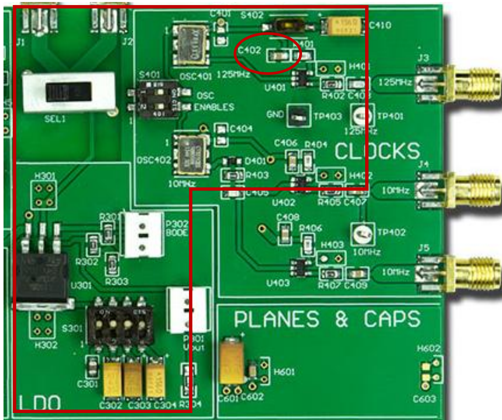
Figure 7: VRTS3 Training board showing the LDO and clock. The Comb signal is injected into capacitor C402, the power rail for the clock oscillator.
