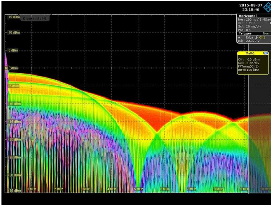
Figures 3: The spectrum when using Mode 3 (100 kHz dithered fundamental).
