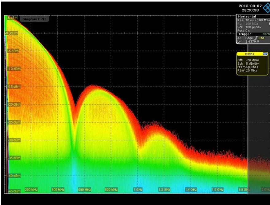
Figure 5: Mode 1 (default sweep mode) includes stepped impulse responses with frequency and width dithering.
